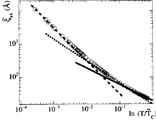
FIG. 1. Renormalized coherence length as a function of the temperature, \bar{\xi}_{ab} (open circles). Parameters appropriate to the fitting of the data on sample IV were used. Various power laws are depicted, in the form \bar{\xi}_{ab} \sim [\ln(T/\bar{T}_c)]^{-\nu} : Gaussian ( \nu=1/2 , full line), critical ( \nu=1 , dashed line), and \nu=2/3 (dotted line).
