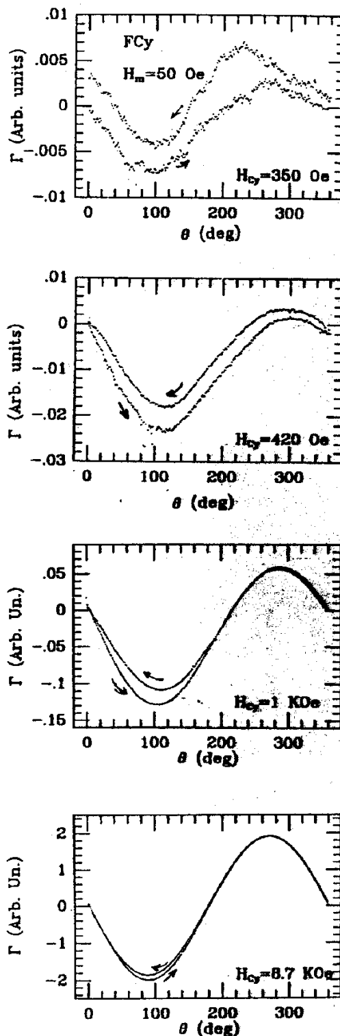
Fig. 4. Torque recordings following protocol 2 for different cycling fields; testing field 50 Oe.
