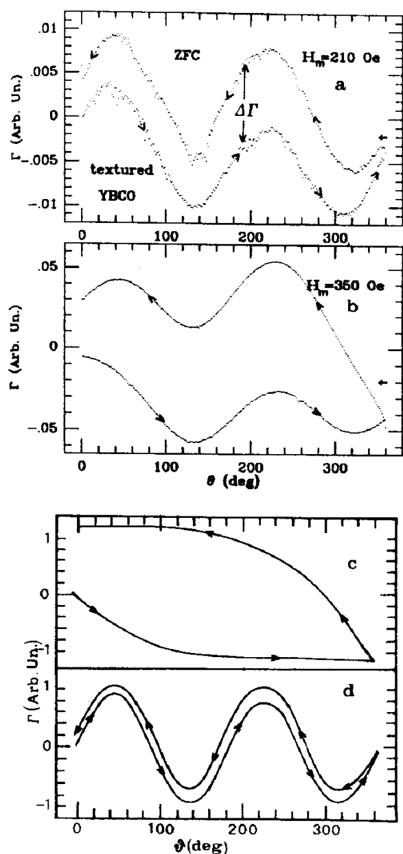
Fig. 1. Torque recordings after protocol 1 from a textured sintered sample (a) for H_m = 210 Oe and (b) H_m = 350 Oe; (c) and (d) are the qualitative behavior for respectively a completely disordered sample and a single crystal.
