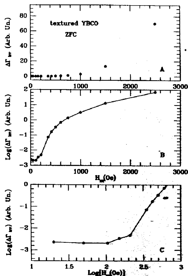
Fig. 2. Peak-to-peak hysteresis vs. H_m in lin-lin (A), lin-log (B) and log-log (C) scales.
